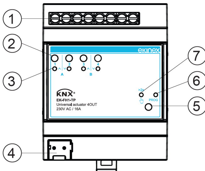
Figure 3 - Switching, display and connection elements for EK-FH1-TP
