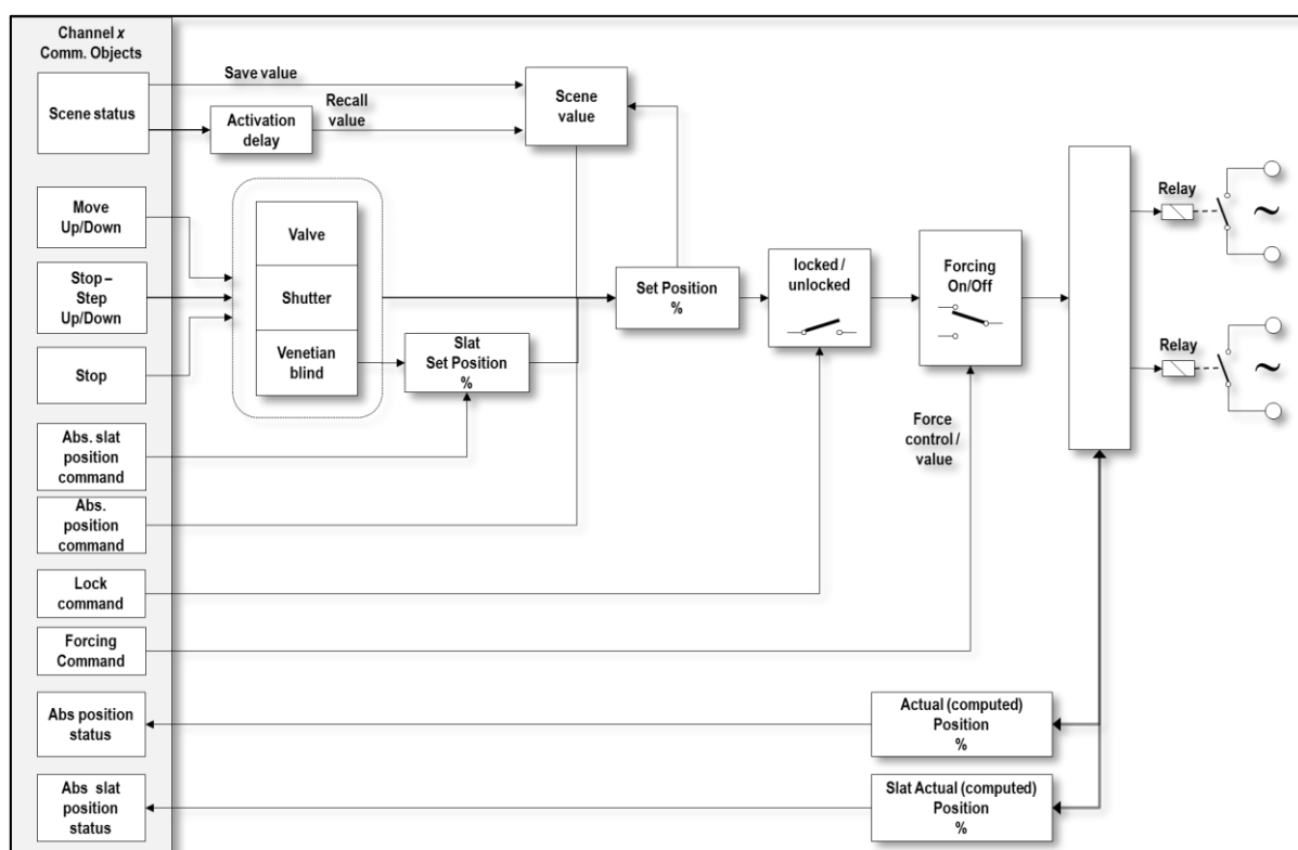
Figure 14 - Functional blocks – Coupled mode (referred to a single output)
